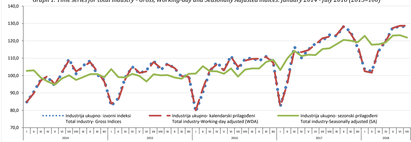
Grafik 1. Vremenska serija industrija ukupno - izvorni, kalendarski i sezonski prilagođeni indeksi: siječanj 2014 - srpanj 2018 (2015=100) Graph 1. Time series for total industry - Gross, Working-day and Seasonally Adjusted indices: January 2014 - July 2018 (2015=100)
