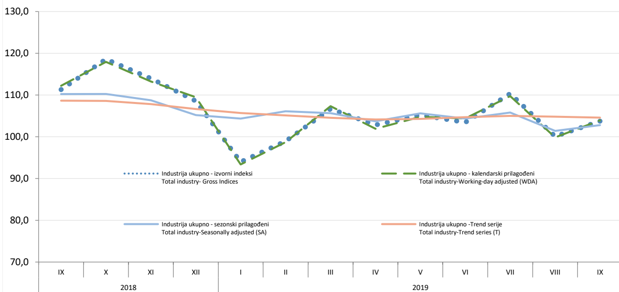
Grafik 1. Mjesečna serija indeksa industrija ukupno - izvorni, kalendarski i sezonski prilagođeni indeksi: septembar 2018 - septembar 2019 (2015=100) Graph 1. Monthly series of industrial indices for total - Gross, Working-day and Seasonally Adjusted indices: September 2018 - September 2019 (2015=100)
