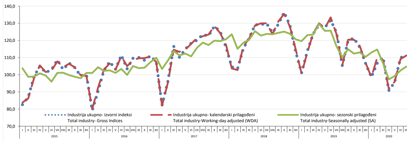
Grafik 1. Vremenska serija industrija ukupno - izvorni, kalendarski i sezonski prilagođeni indeksi: januar 2015 - juli 2020 (2015=100) Graph 1. Time series for total industry - Gross, Working-day and Seasonally Adjusted indices: January 2015 - July 2020 (2015=100)
