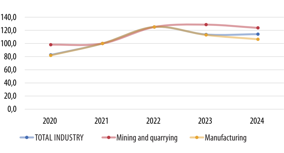
Industry turnover index in BiH by type of market, by year (2021=100)
