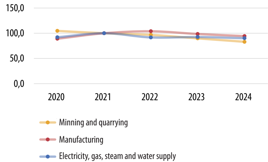
Annual gross volume index of industrial production by activity section and main industrial groups (2021=100)
