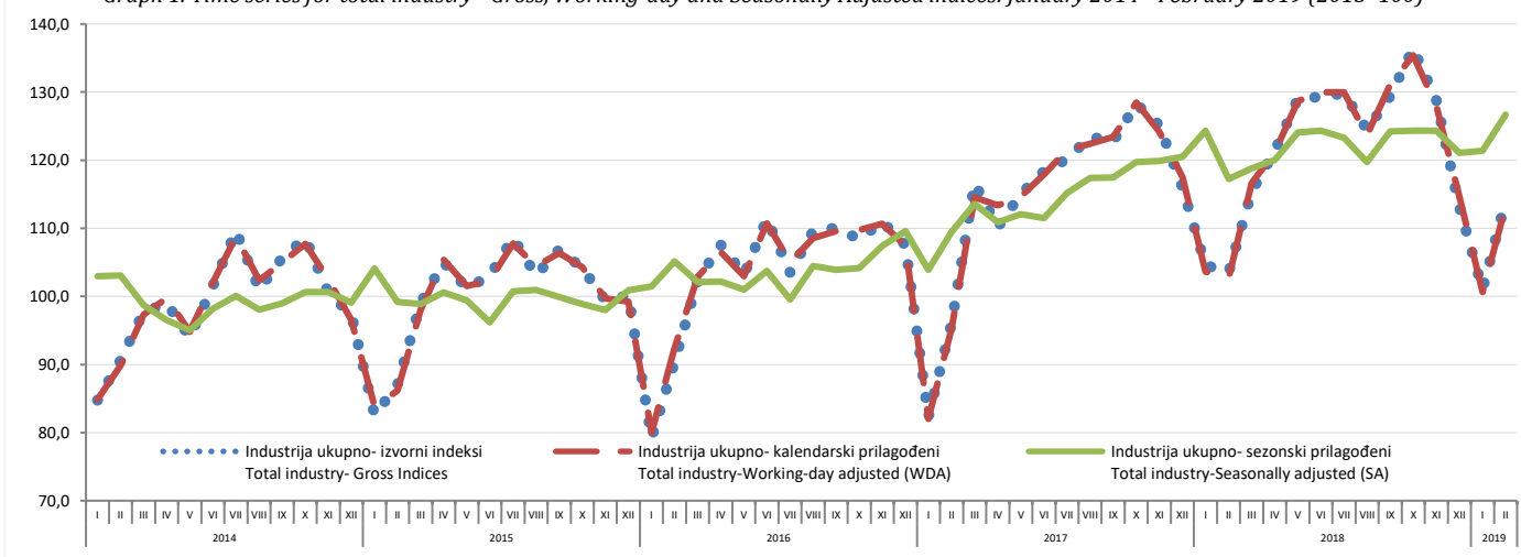
Grafik 1. Vremenska serija industrija ukupno - izvorni, kalendarski i sezonski prilagođeni indeksi: siječanj 2014 - veljača 2019 (2015=100) Graph 1. Time series for total industry - Gross, Working-day and Seasonally Adjusted indices: January 2014 - February 2019 (2015=100)
