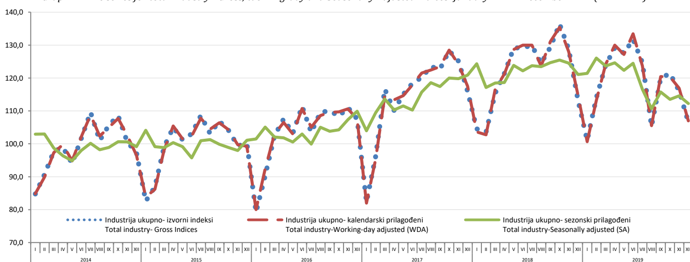
Grafik 1. Vremenska serija industrija ukupno - izvorni, kalendarski i sezonski prilagođeni indeksi: siječanj 2014 - prosinac 2019 (2015=100) Graph 1. Time series for total industry - Gross, Working-day and Seasonally Adjusted indices: January 2014 - December 2019 (2015=100)
