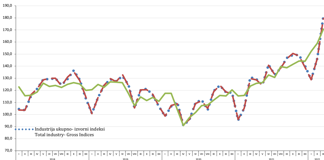
Grafik 1. Vremenska serija industrija ukupno - izvorni, kalendarski i sezonski prilagođeni indeksi: siječanj 2018. - ožujak 2022. (2015=100) Graph 1. Time series for total industry - Gross, Working-day and Seasonally Adjusted indices: January 2018 - March 2022 (2015=100)
