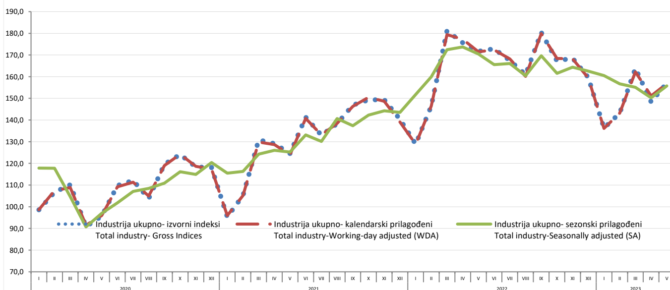
Grafik 1. Vremenska serija industrija ukupno - izvorni, kalendarski i sezonski prilagođeni indeksi: januar 2020 - maj 2023 (2015=100) Graph 1. Time series for total industry - Gross, Working-day and Seasonally Adjusted indices: January 2020 - May 2023 (2015=100)
