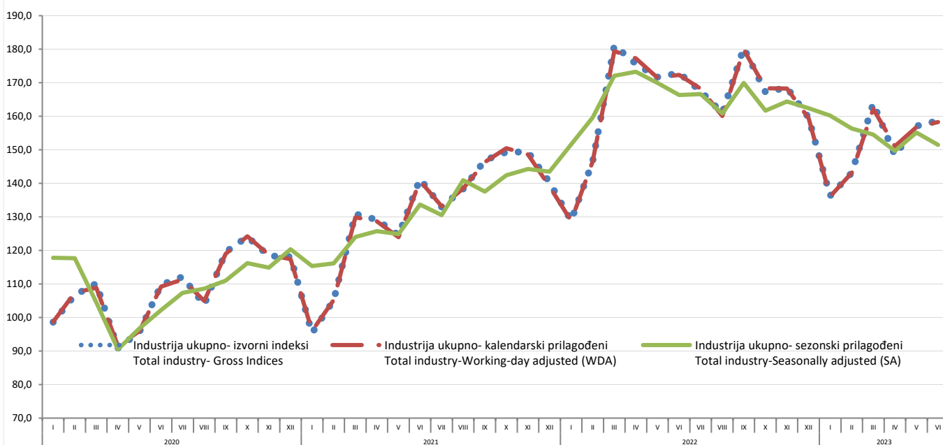
Grafik 1. Vremenska serija industrija ukupno - izvorni, kalendarski i sezonski prilagođeni indeksi: januar 2020. - juni 2023. (2015=100) Graph 1. Time series for total industry - Gross, Working-day and Seasonally Adjusted indices: January 2020 - June 2023 (2015=100)
