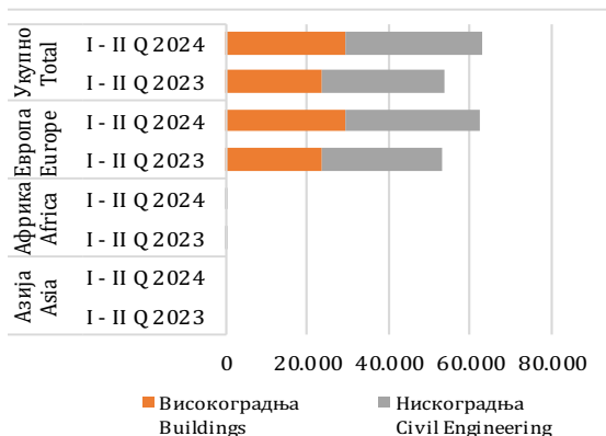
Figure 1 THE VALUE OF PERFORMED CONSTRUCTION WORKS ABROAD, JANUARY – JUNE 2024
