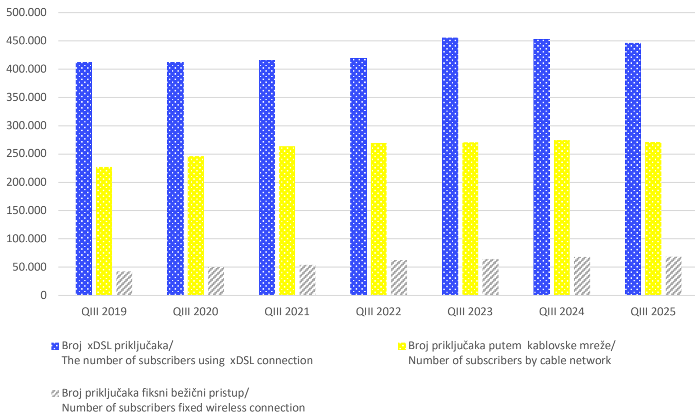
Grafikon 3.2. Tip priključaka pristupa internetu putem fiksne mreže Graph 3.2 Type connectors of Internet access connections via the fixed network
