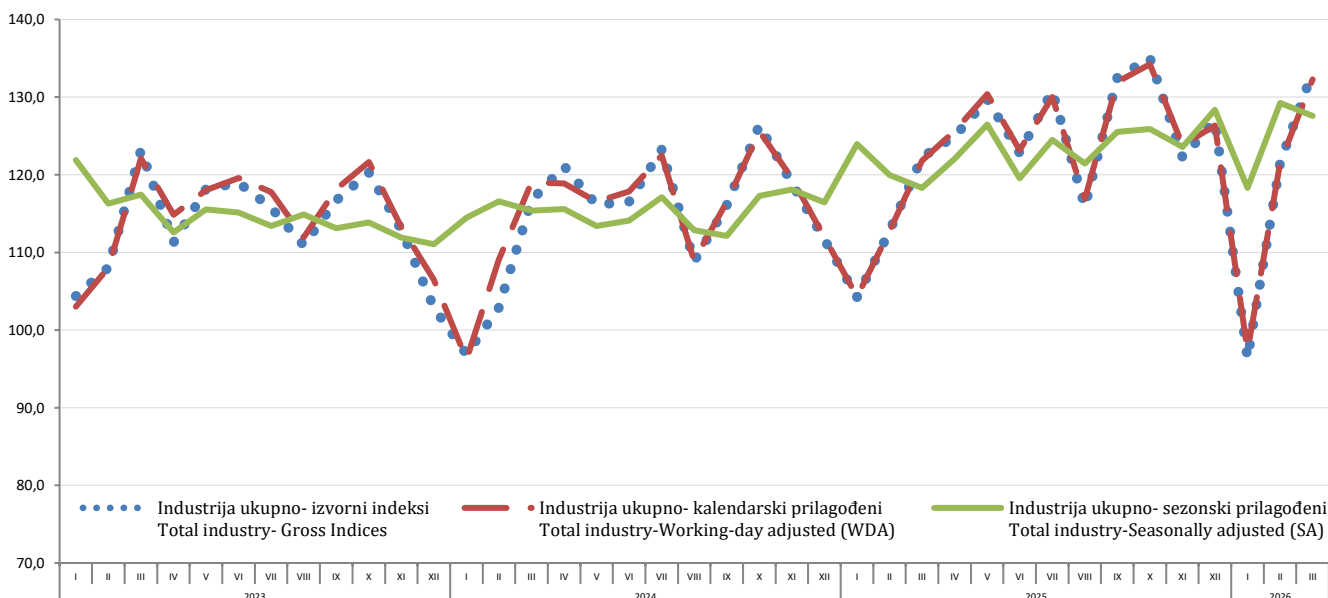
Grafik 1. Vremenska serija industrija ukupno - izvorni, kalendarski i sezonski prilagođeni indeksi: siječanj 2023 - ožujak 2026 (2021=100) Graph 1. Time series for total industry - Gross, Working-day and Seasonally Adjusted indices: January 2023 - March 2026 (2021=100)
